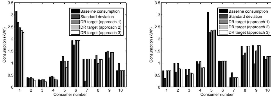
Figure 6: Comparison of DR target consumptions for consumers during during time slots t = 13 (left) and t = 22 (right) using the first three optimization approaches. The baseline and standard deviation based on historical data are also shown for reference. Note that at t = 13 , while consumers with small baseline and standard deviation (e.g. 2 and 4) are never targeted in the deterministic case (approach 1), they can be targeted in the stochastic case (approach 2) due to their higher participation probabilities.
